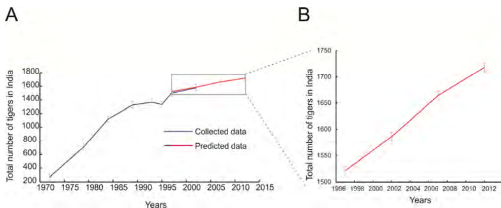
Fig. 6. Growth of tigers with predictions. A. The plot shows the nature / pattern of statistical data for tiger population in India from 1972 - 2002 (blue line) and an extended prediction (red line) of the curve to 2012 using continuous growth model simulator. The model assumes a 10% standard deviation shown by the error bar. B. The plot shows the enlarged curve of predicted piece-wise continuous growth of tiger populations in India
